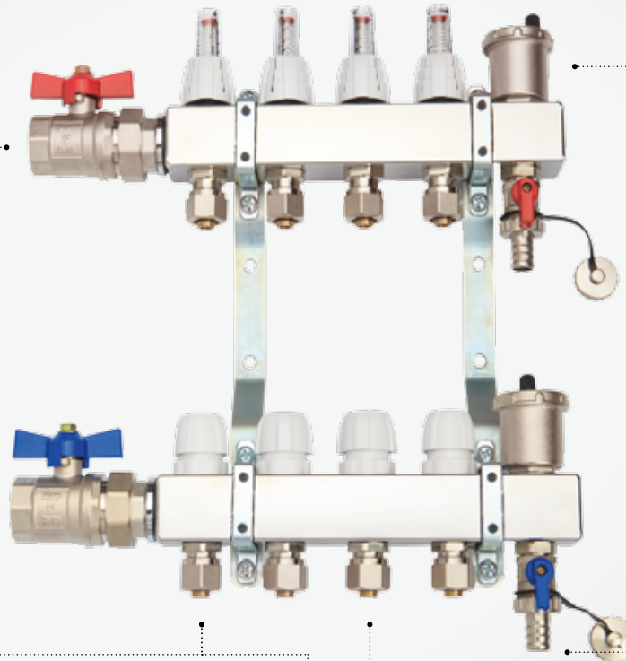
Control valve with flowmeter
