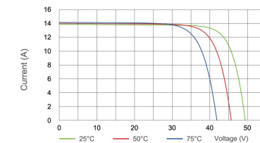
Power voltage current curve at different temperature
