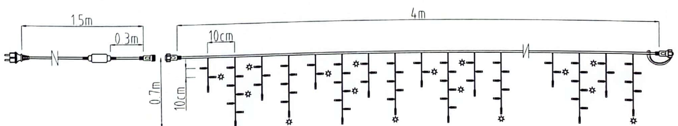
ENO 200L/E Icicle Lights: 4m x 0.7m 20% Flash/Steady Flash Led 2/3; 4/7; 1/4; 6/6
